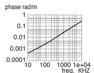
High frequency characteristics of Part No.2964 and #2965. 品番2964と2965の高周波特性。
