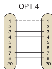
FOR ASYNCHRONOUS MODEM
