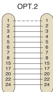
FOR JIS C6361 MODEM ( M1,2,3,4 ALL COVERED )
