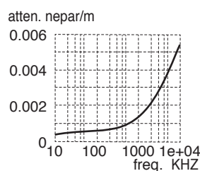
High frequency characteristics of Part No.2964 and #2965. 品番2964と2965の高周波特性。
