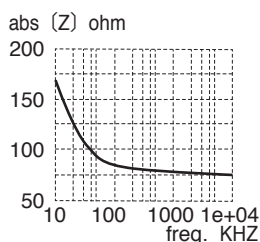
High frequency characteristics of Part No.2964 and #2965. 品番2964と2965の高周波特性。
