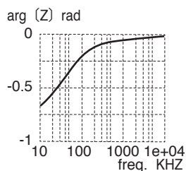
High frequency characteristics of Part No.2964 and #2965. 品番2964と2965の高周波特性。
